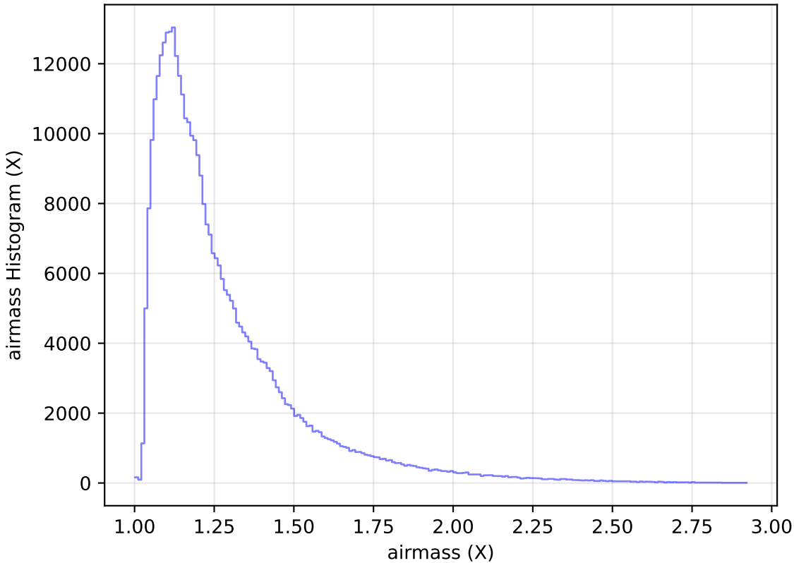
too_elab_r16_d3_giz_v3.4_10yrs All sky y band: airmass Histogram
