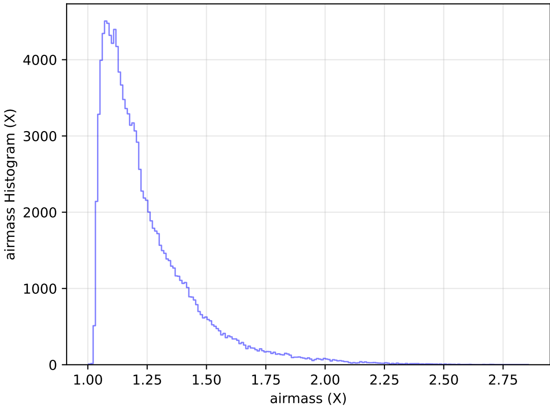
too_elab_r16_d3_giz_v3.4_10yrs All sky u band: airmass Histogram
