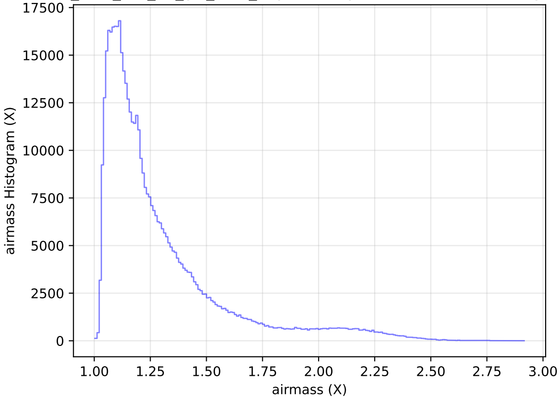
too_elab_r16_d3_giz_v3.4_10yrs All sky r band: airmass Histogram
