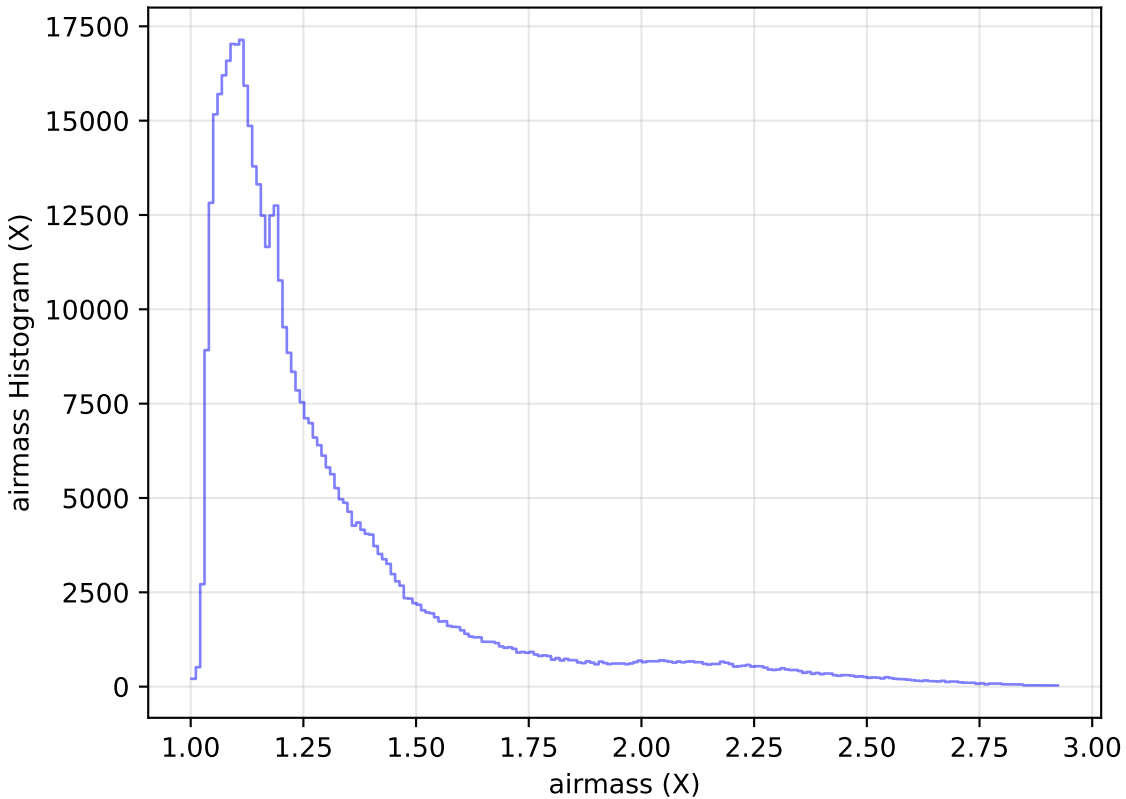
too_elab_r16_d3_giz_v3.4_10yrs All sky i band: airmass Histogram
