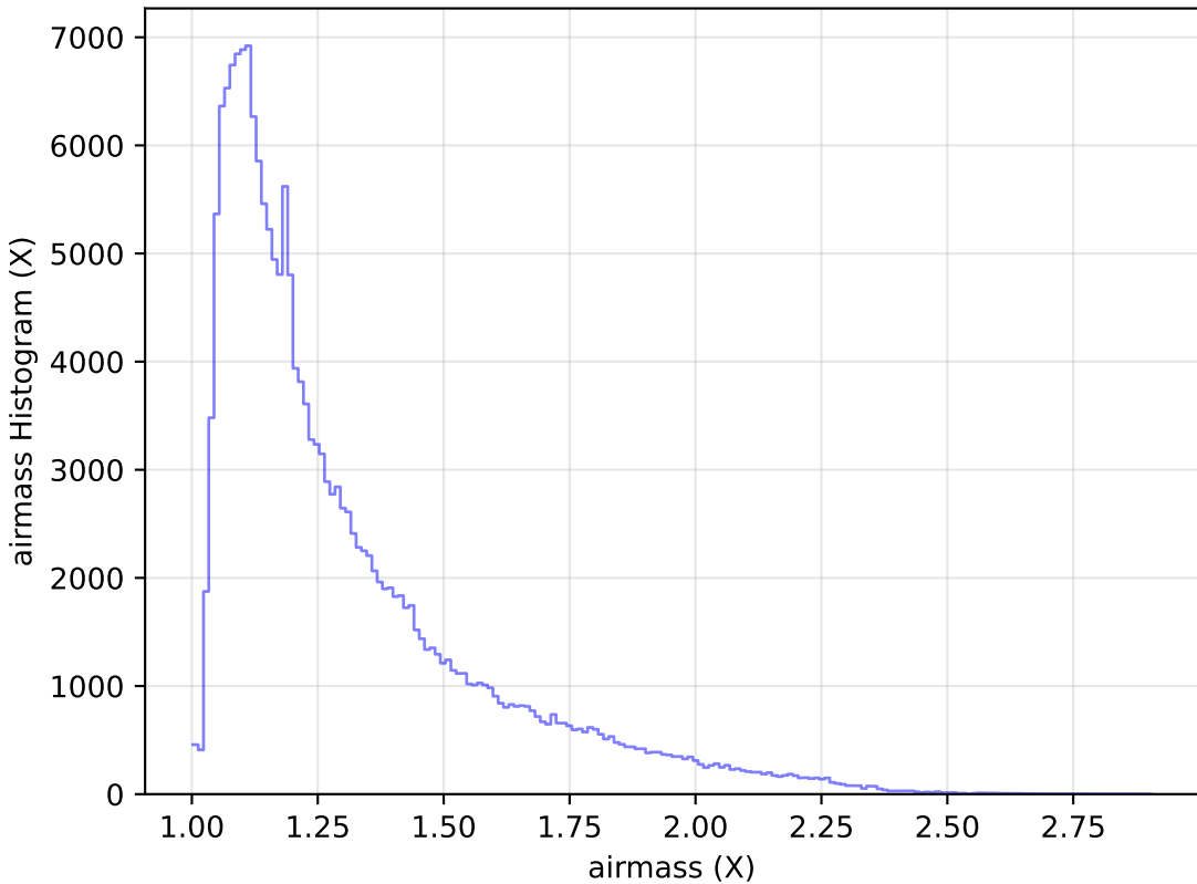
too_elab_r16_d3_giz_v3.4_10yrs All sky g band: airmass Histogram
