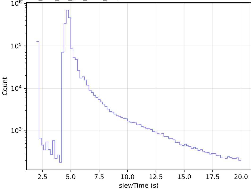
too_elab_r16_d3_giz_v3.4_10yrs All visits: Zoom Slew Time Histogram
