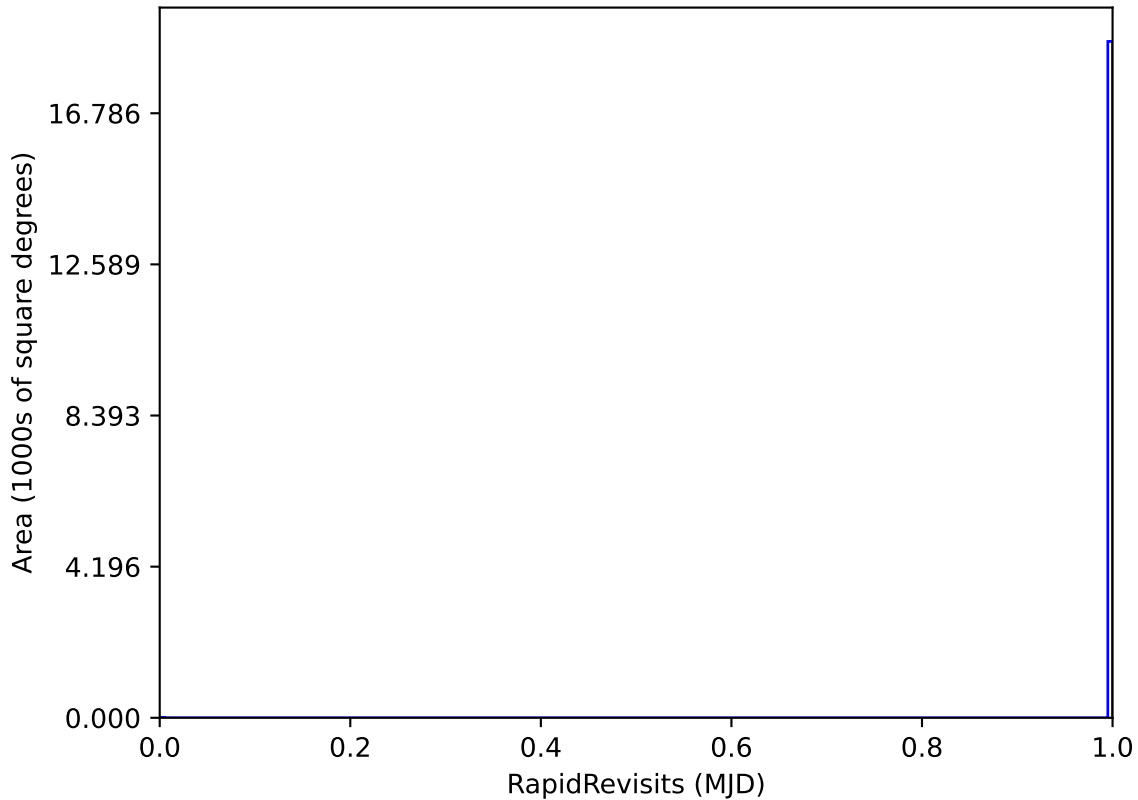
too_elab_r16_d3_giz_v3.4_10yrs WFD: RapidRevisits
