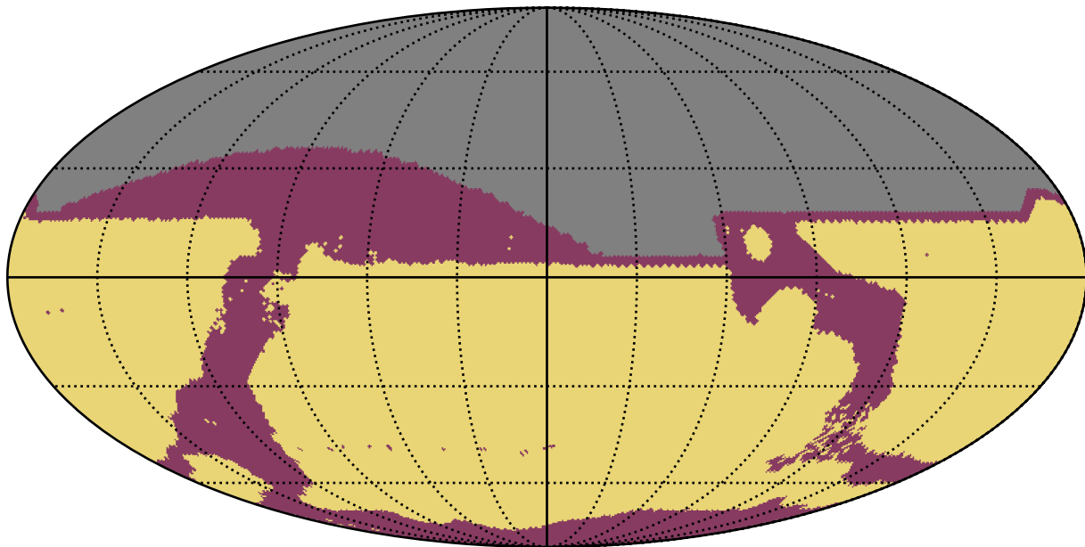
too_elab_r16_d3_giz_v3.4_10yrs All sky: RapidRevisits
