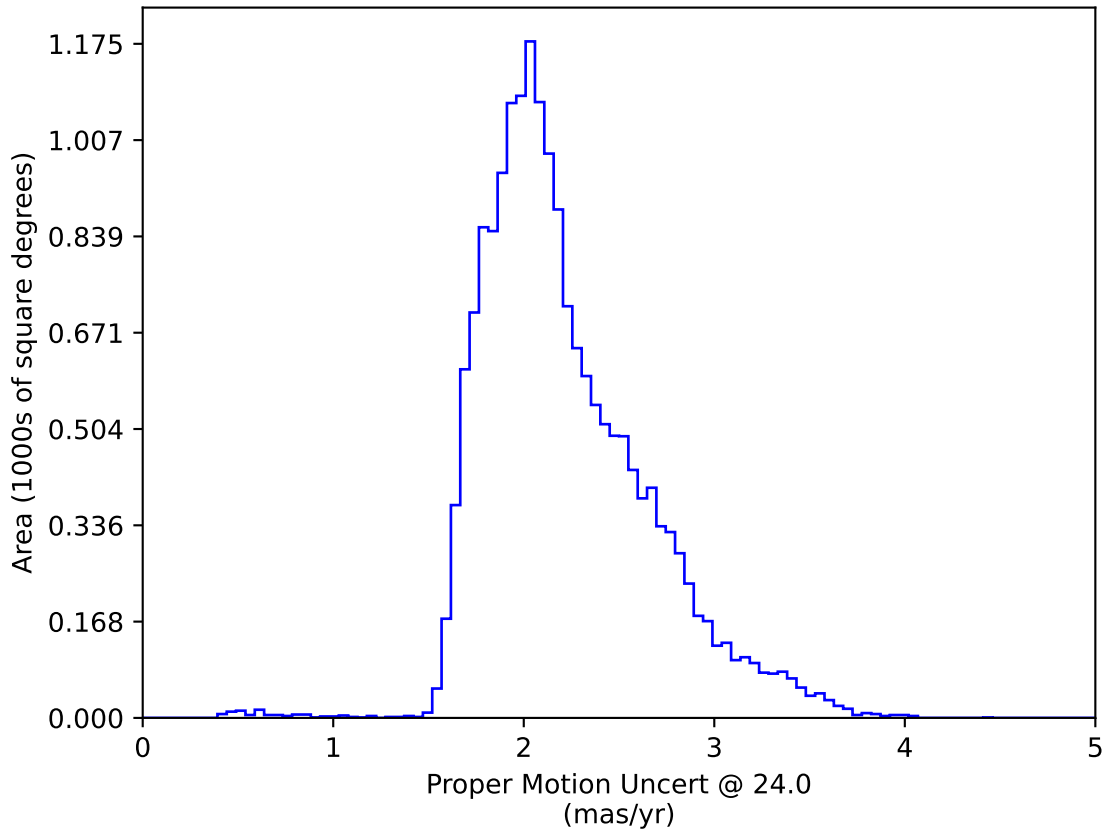
too_elab_r16_d3_giz_v3.4_10yrs WFD: Proper Motion Uncert @ 24.0
