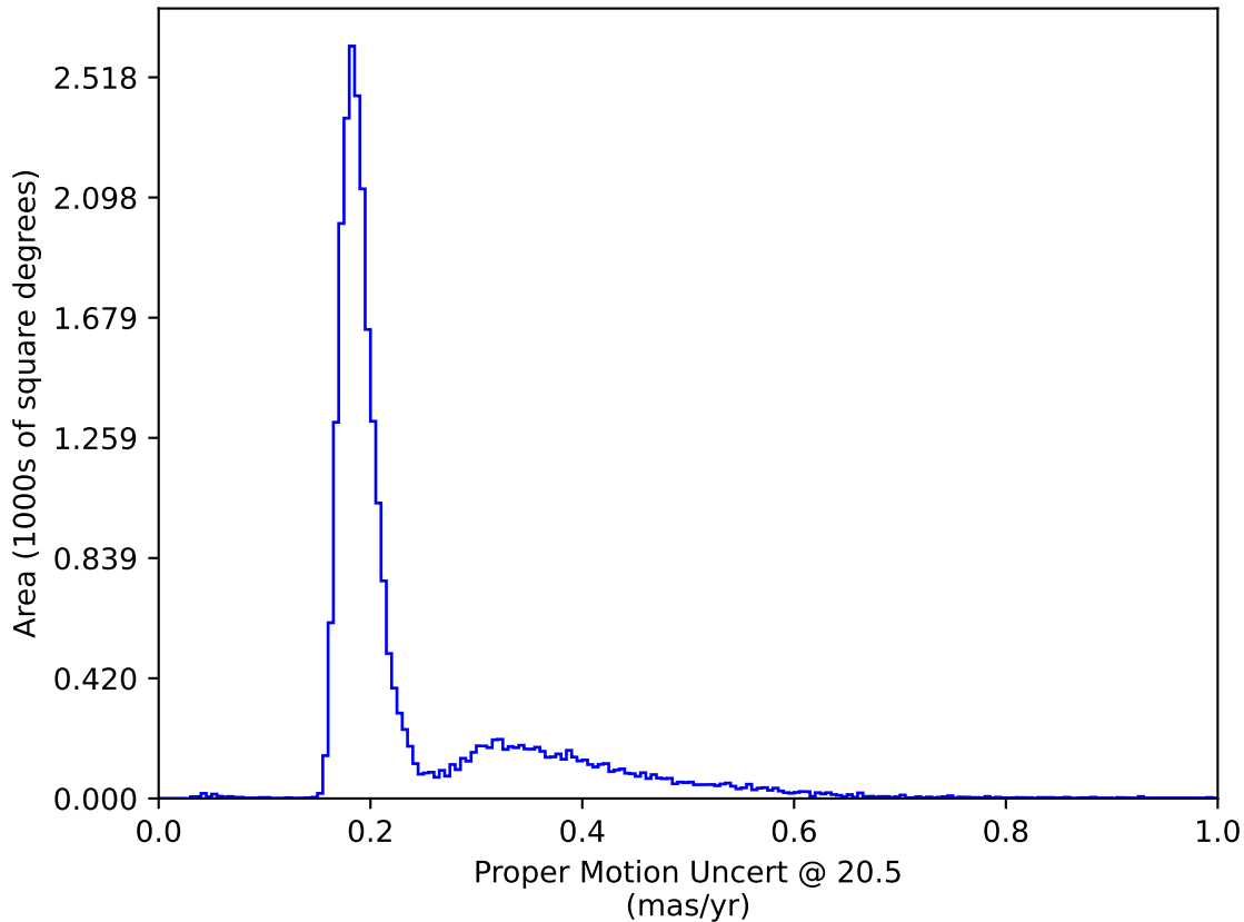
too_elab_r16_d3_giz_v3.4_10yrs All sky: Proper Motion Uncert @ 20.5
