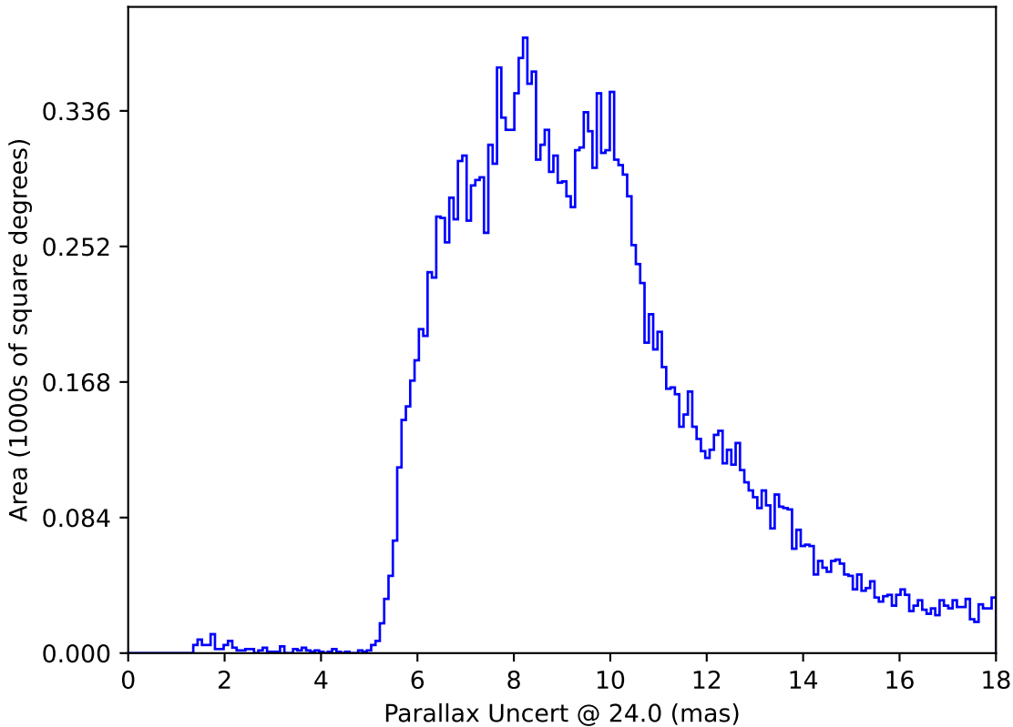
too_elab_r16_d3_giz_v3.4_10yrs All sky: Parallax Uncert @ 24.0
