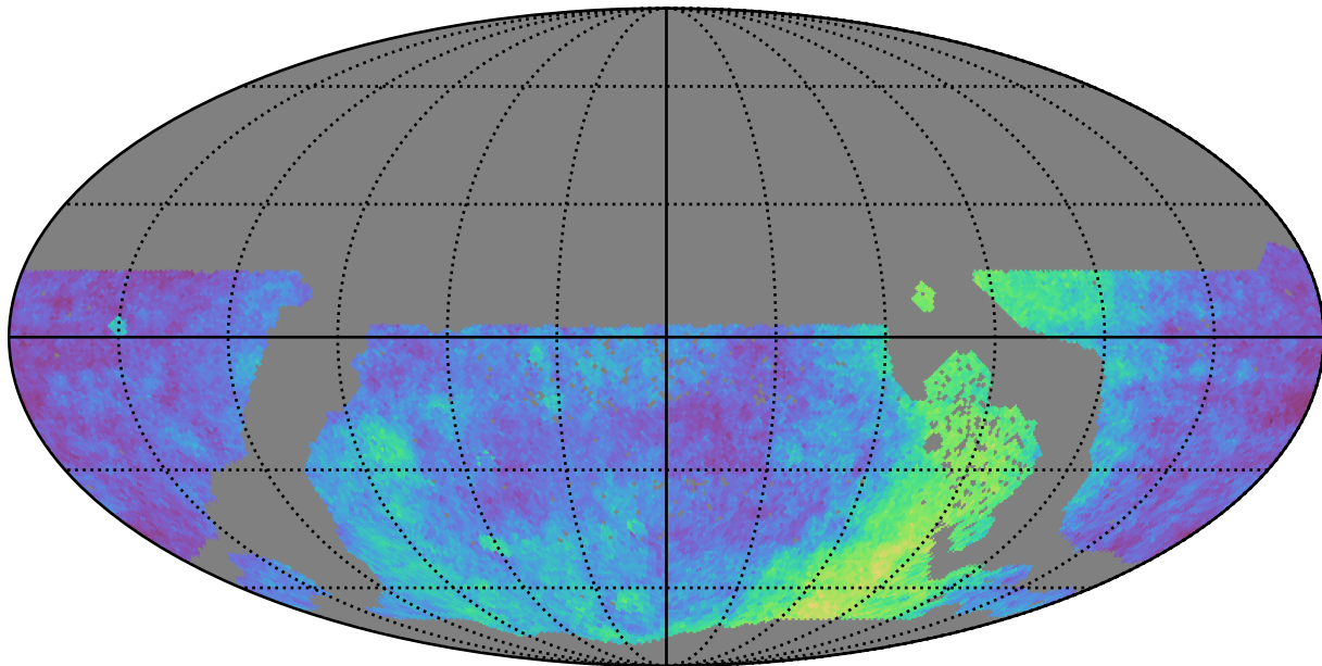
too_elab_r16_d3_giz_v3.4_10yrs WFD: Parallax Coverage @ 24.0
