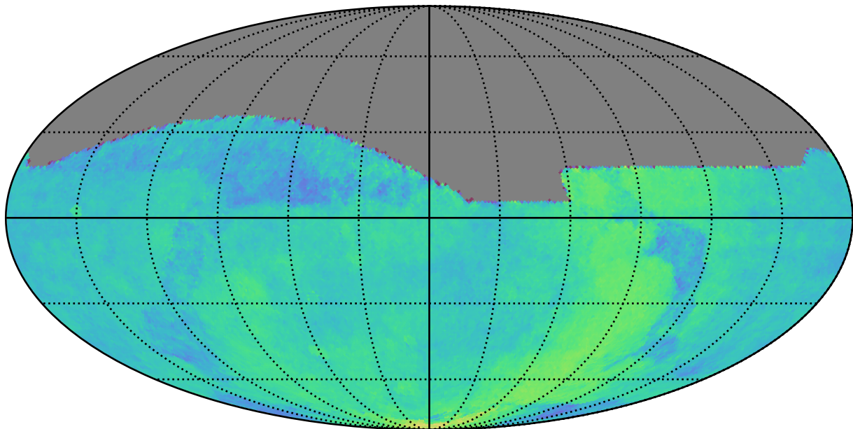
too_elab_r16_d3_giz_v3.4_10yrs All sky: Parallax Coverage @ 24.0
