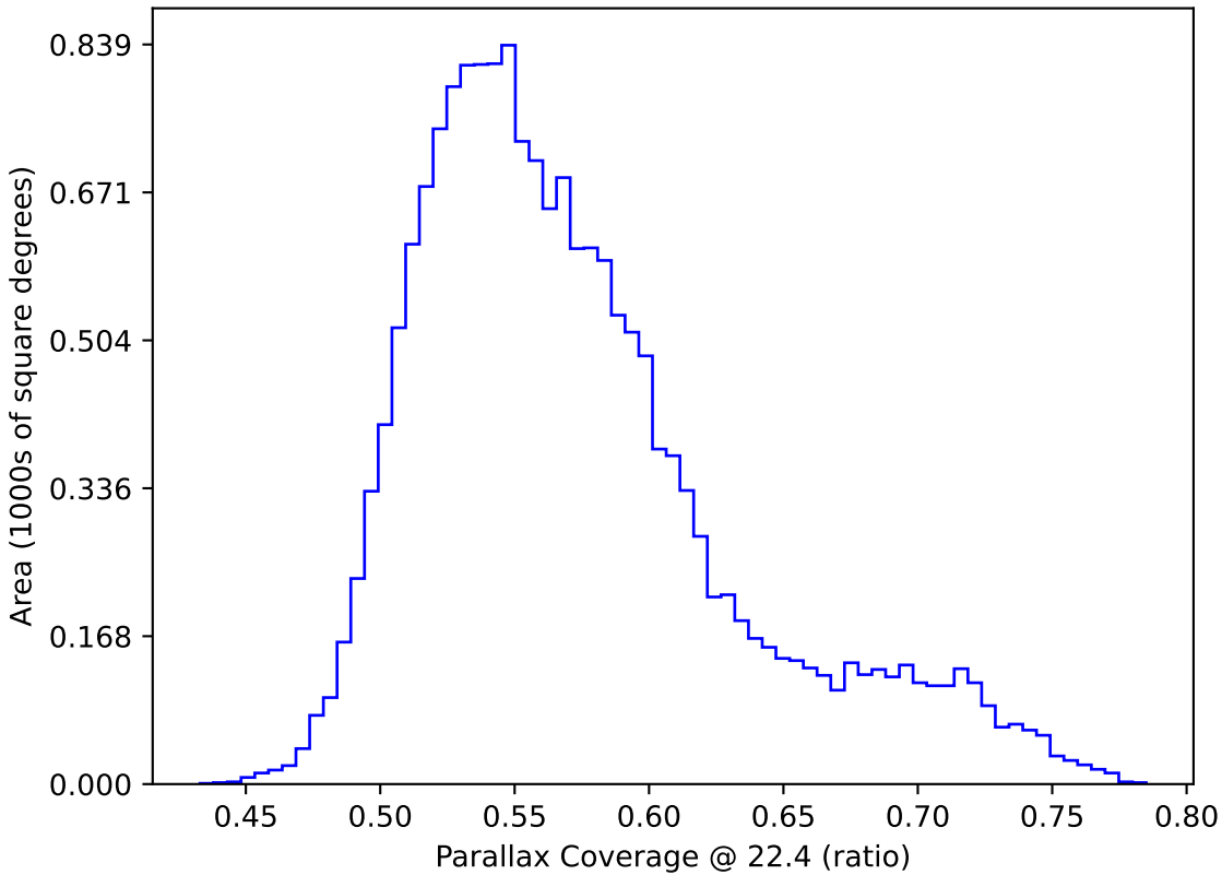
too_elab_r16_d3_giz_v3.4_10yrs WFD: Parallax Coverage @ 22.4
