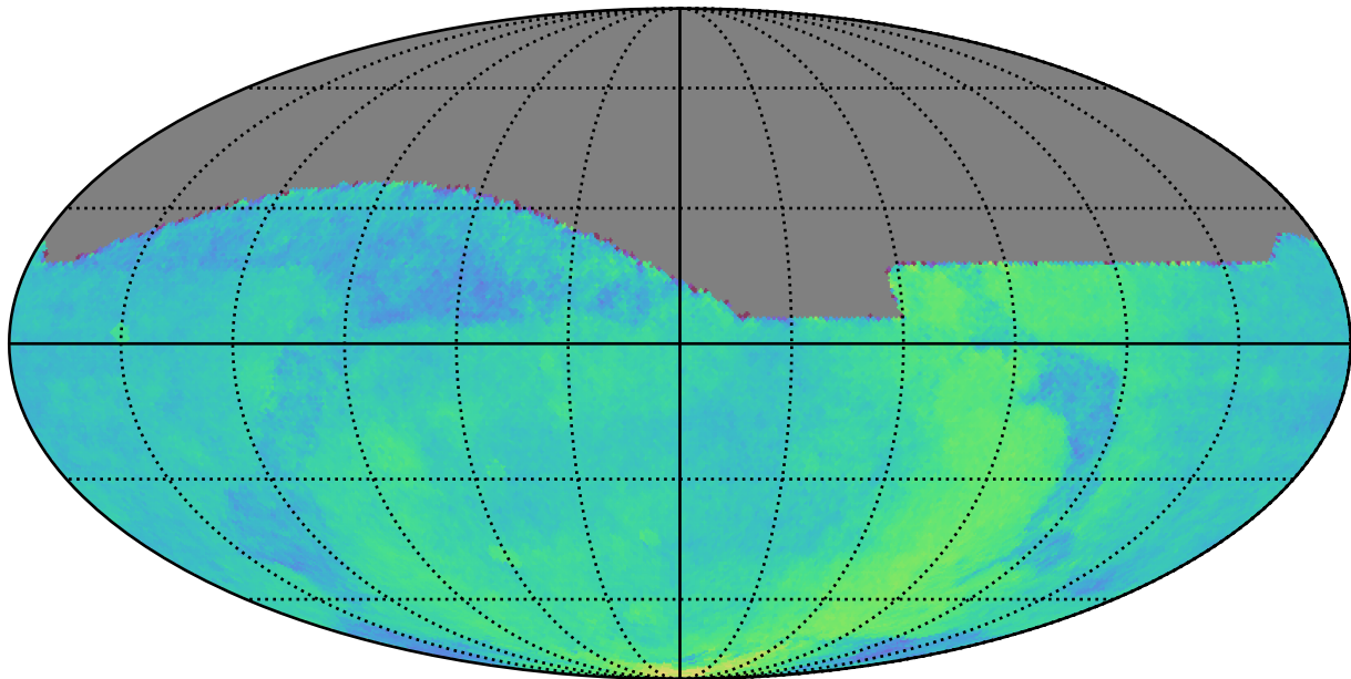
too_elab_r16_d3_giz_v3.4_10yrs All sky: Parallax Coverage @ 22.4
