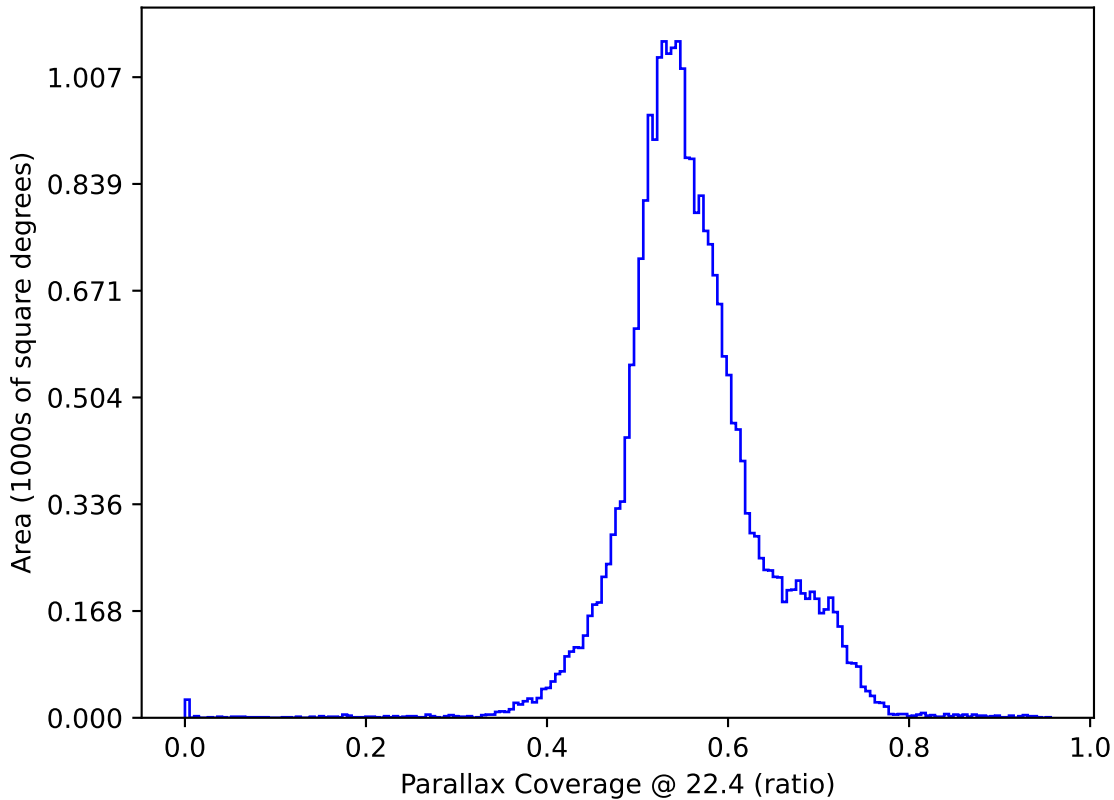
too_elab_r16_d3_giz_v3.4_10yrs All sky: Parallax Coverage @ 22.4
