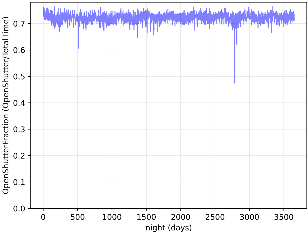
too_elab_r16_d3_giz_v3.4_10yrs Per night: OpenShutterFraction
