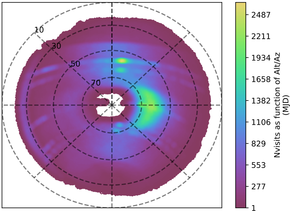
too_elab_r16_d3_giz_v3.4_10yrs r band: Nvisits as function of Alt/Az
