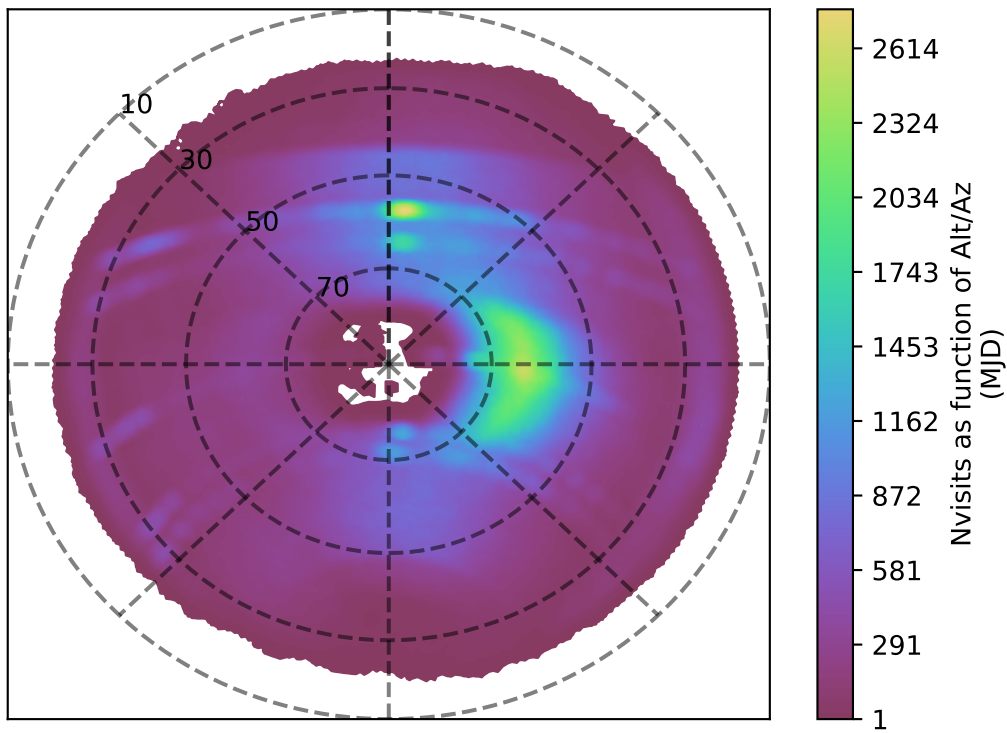
too_elab_r16_d3_giz_v3.4_10yrs i band: Nvisits as function of Alt/Az
