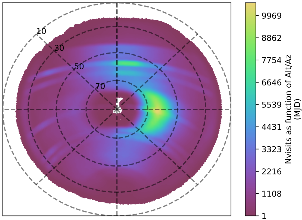
too_elab_r16_d3_giz_v3.4_10yrs all bands: Nvisits as function of Alt/Az
