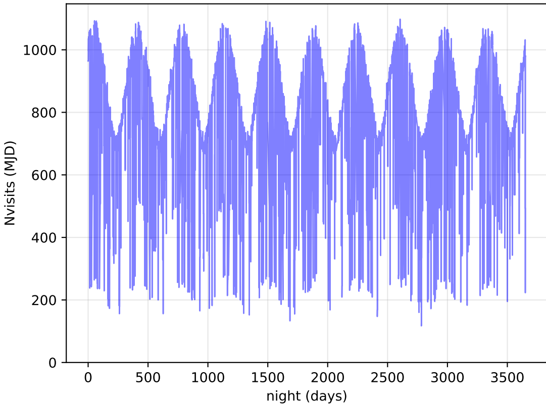
too_elab_r16_d3_giz_v3.4_10yrs All visits: Nvisits
