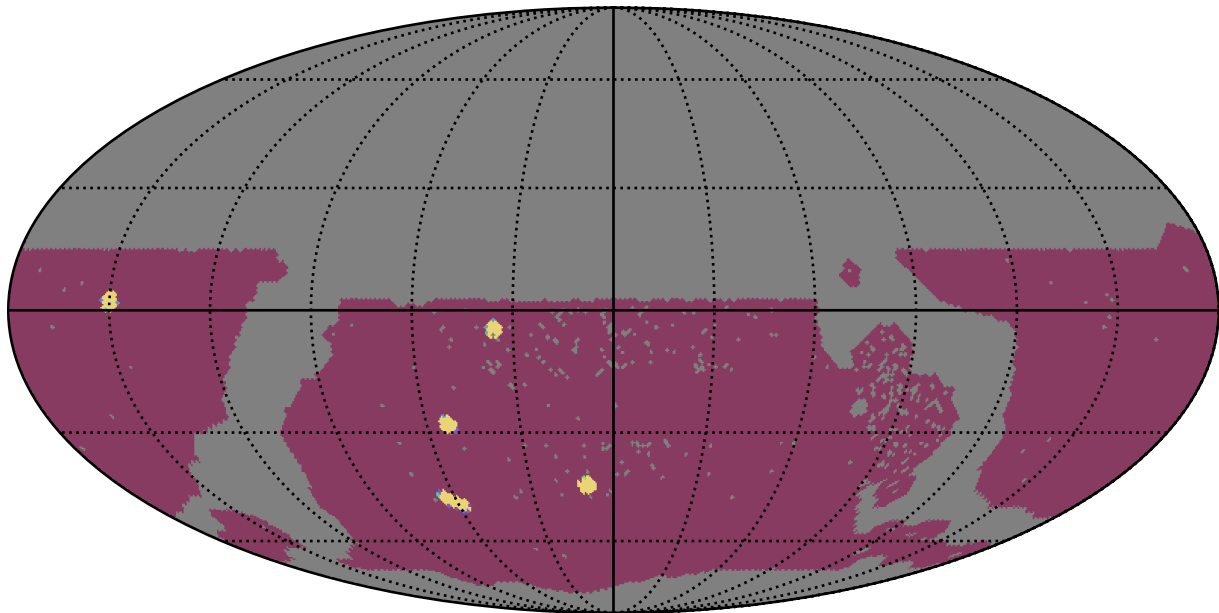
too_elab_r16_d3_giz_v3.4_10yrs WFD: NumberOfQuickRevisits
