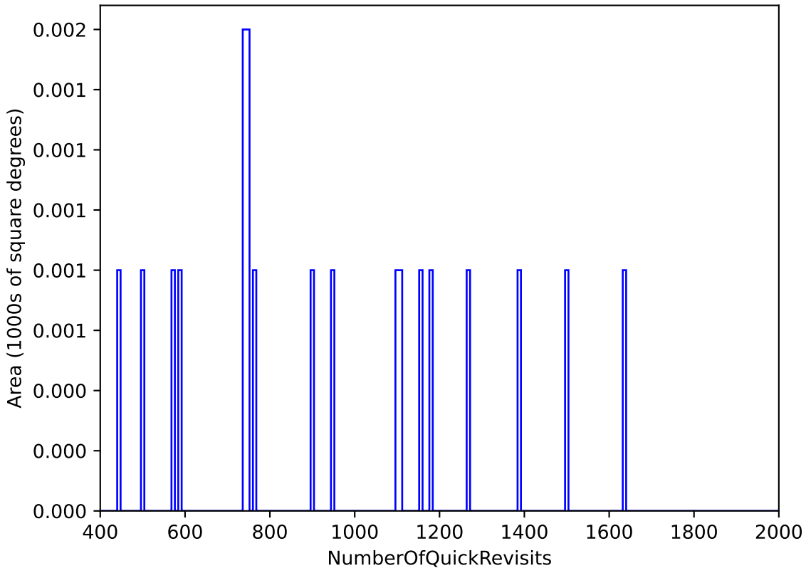
too_elab_r16_d3_giz_v3.4_10yrs WFD: NumberOfQuickRevisits
