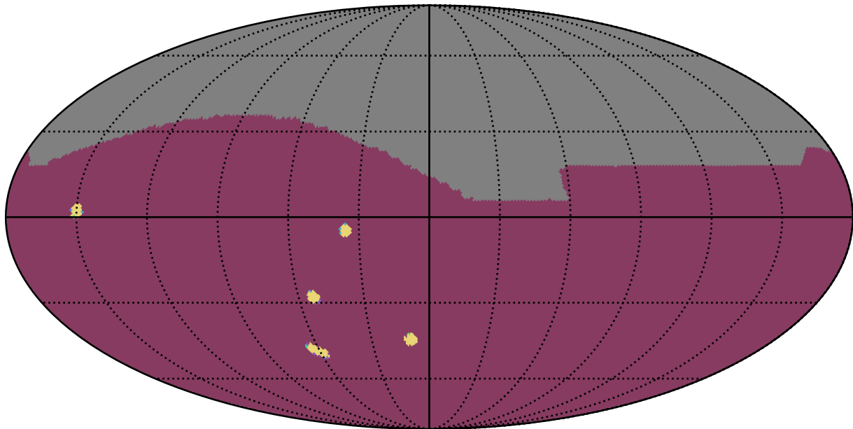
too_elab_r16_d3_giz_v3.4_10yrs All sky: NumberOfQuickRevisits
