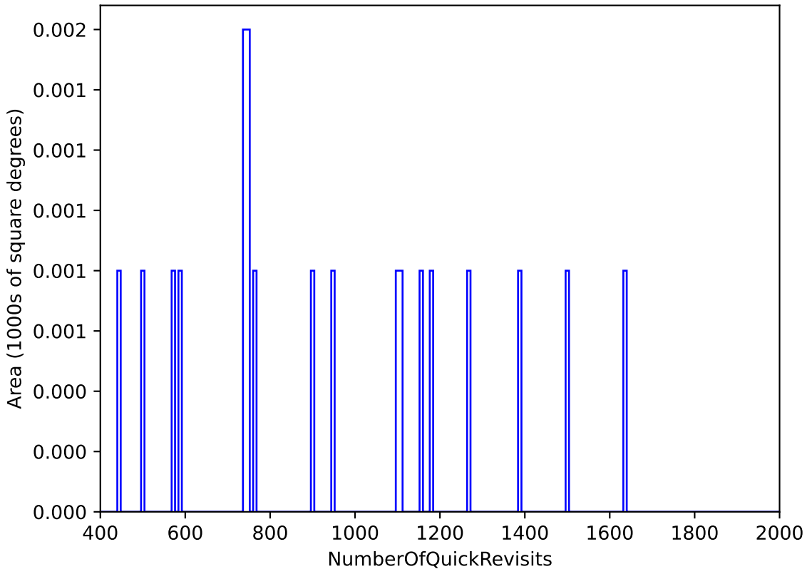
too_elab_r16_d3_giz_v3.4_10yrs All sky: NumberOfQuickRevisits
