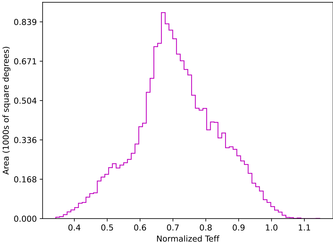
too_elab_r16_d3_giz_v3.4_10yrs WFD z band: Normalized Teff
