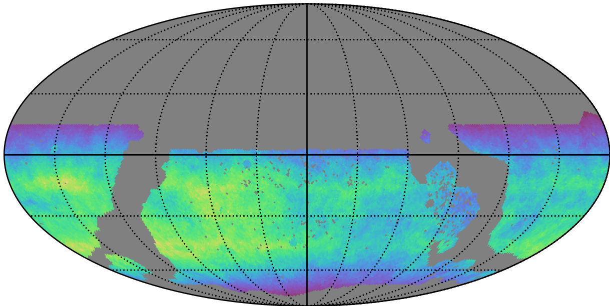
too_elab_r16_d3_giz_v3.4_10yrs WFD y band: Normalized Teff
