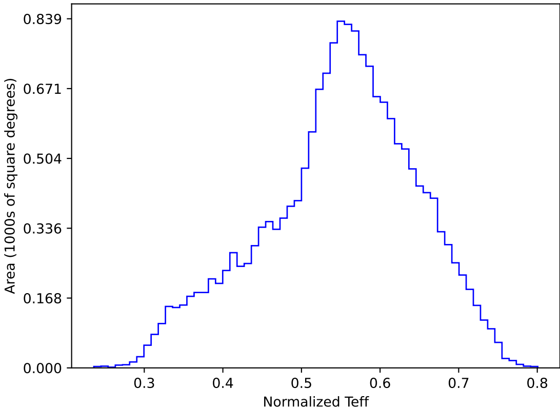
too_elab_r16_d3_giz_v3.4_10yrs WFD y band: Normalized Teff
