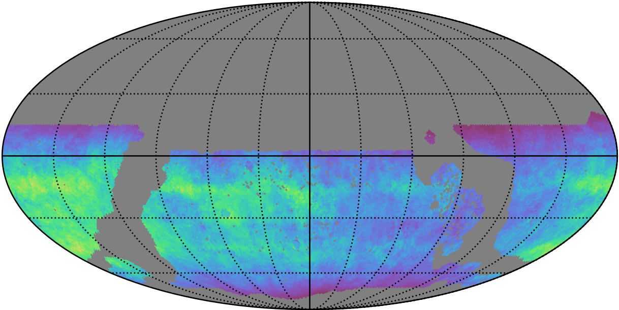
too_elab_r16_d3_giz_v3.4_10yrs WFD u band: Normalized Teff
