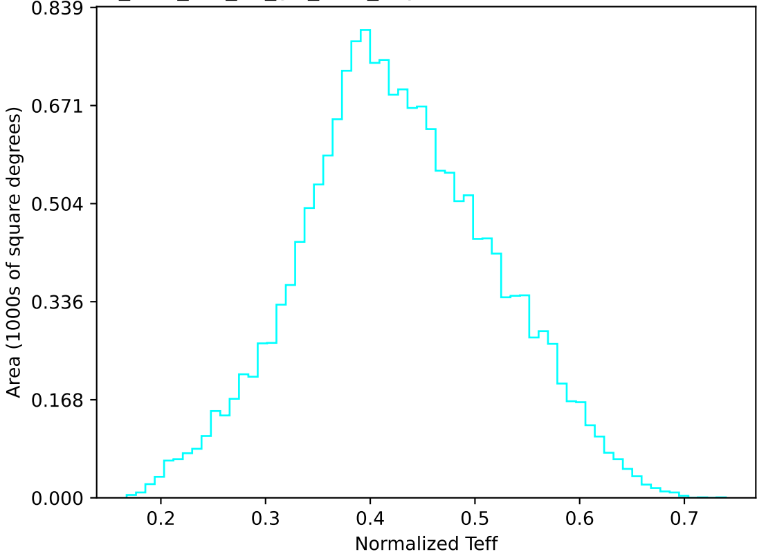
too_elab_r16_d3_giz_v3.4_10yrs WFD u band: Normalized Teff
