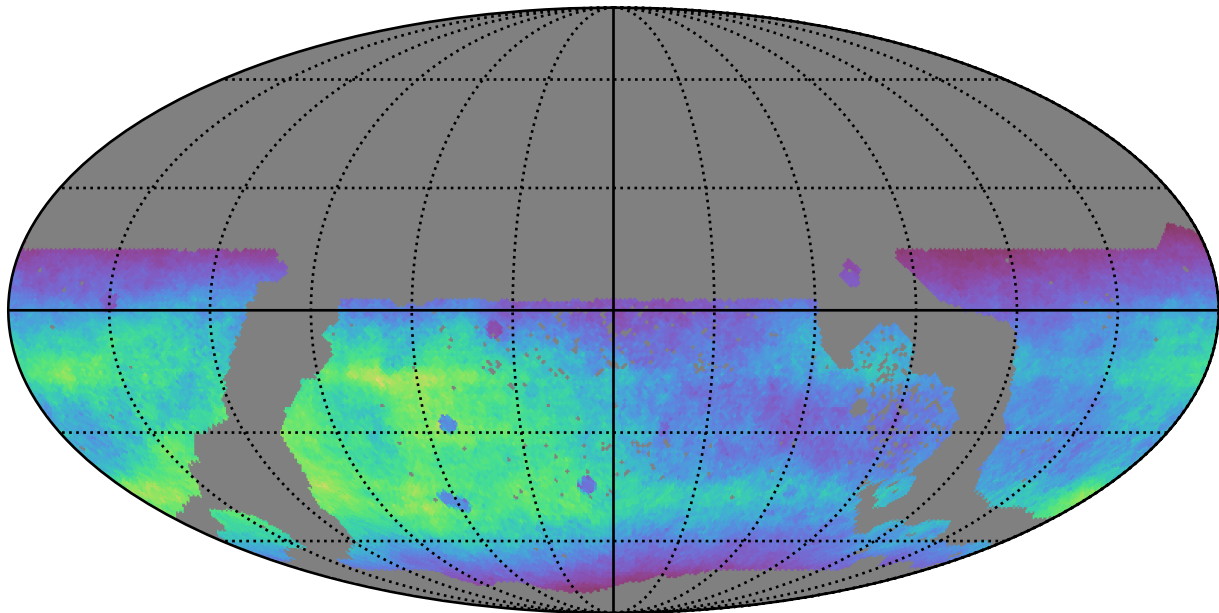
too_elab_r16_d3_giz_v3.4_10yrs WFD r band: Normalized Teff
