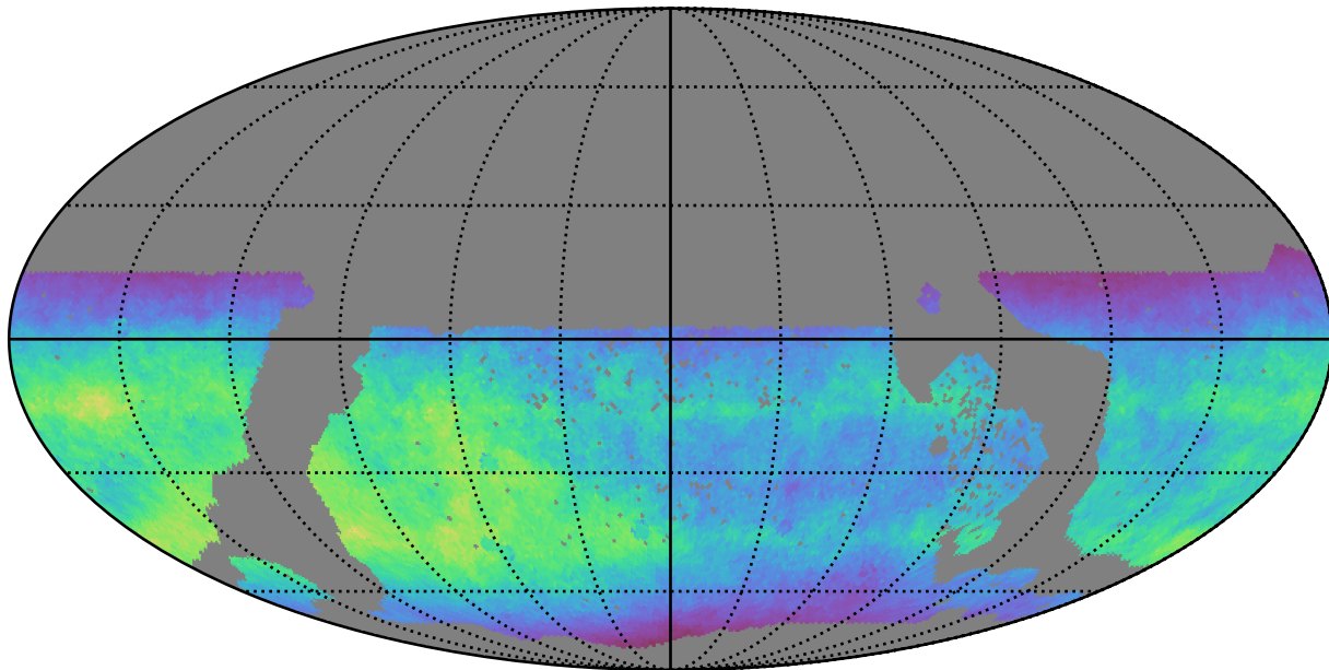
too_elab_r16_d3_giz_v3.4_10yrs WFD i band: Normalized Teff
