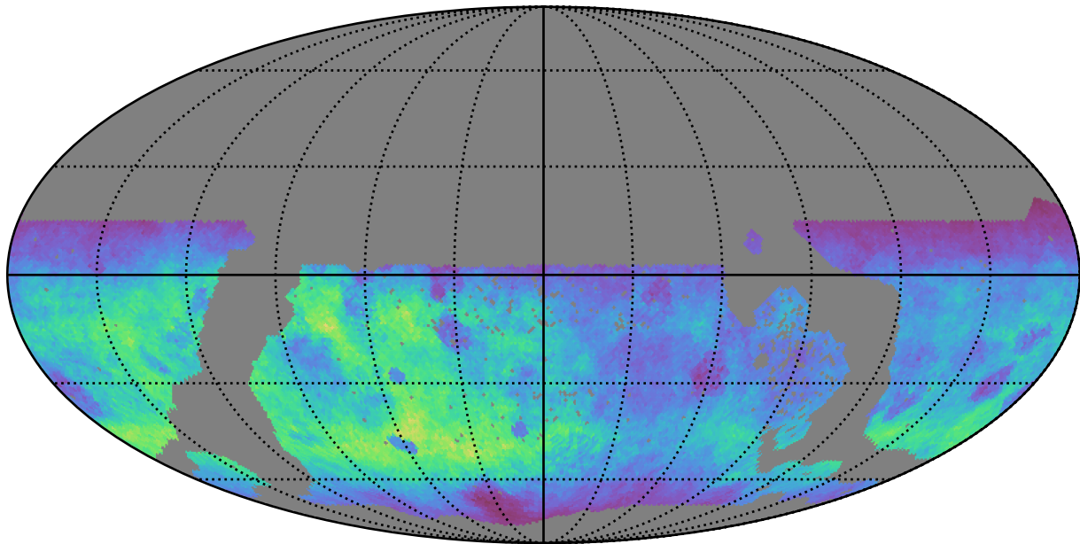
too_elab_r16_d3_giz_v3.4_10yrs WFD g band: Normalized Teff
