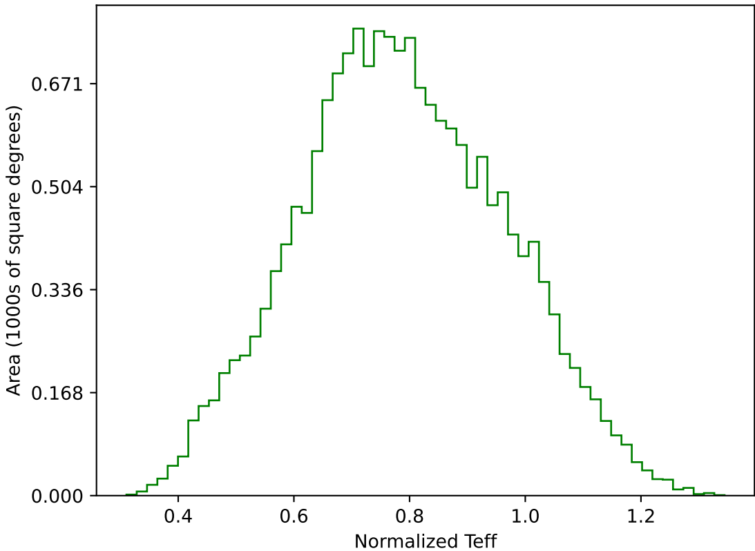
too_elab_r16_d3_giz_v3.4_10yrs WFD g band: Normalized Teff
