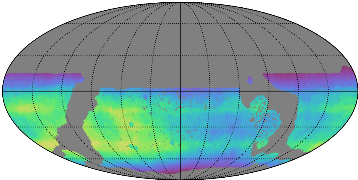
too_elab_r16_d3_giz_v3.4_10yrs WFD all bands: Normalized Teff
