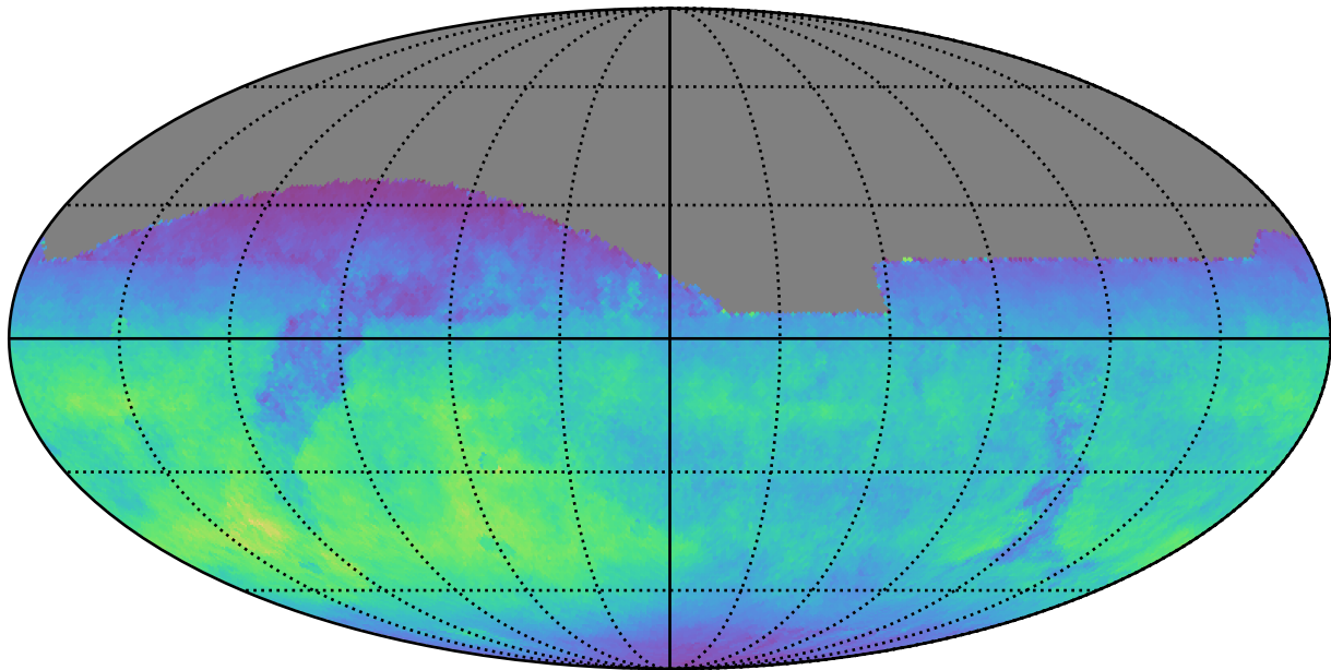
too_elab_r16_d3_giz_v3.4_10yrs All sky z band: Normalized Teff
