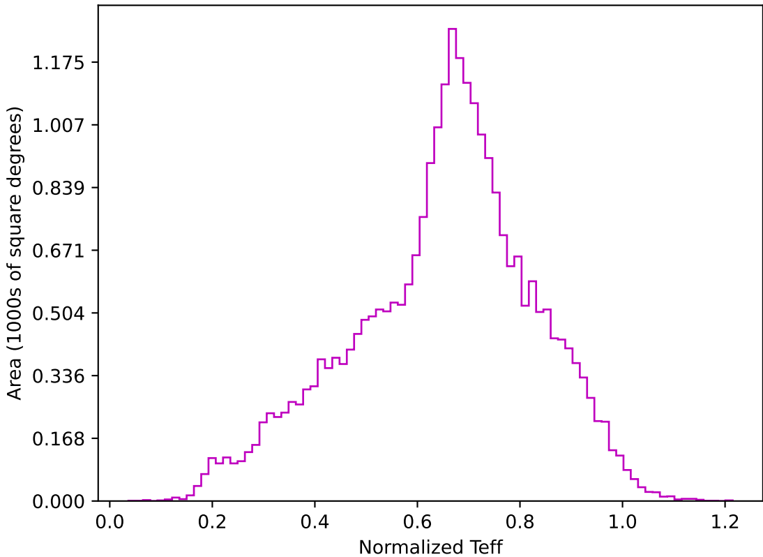
too_elab_r16_d3_giz_v3.4_10yrs All sky z band: Normalized Teff
