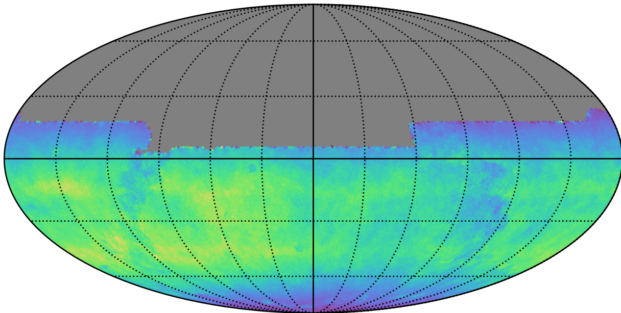
too_elab_r16_d3_giz_v3.4_10yrs All sky y band: Normalized Teff
