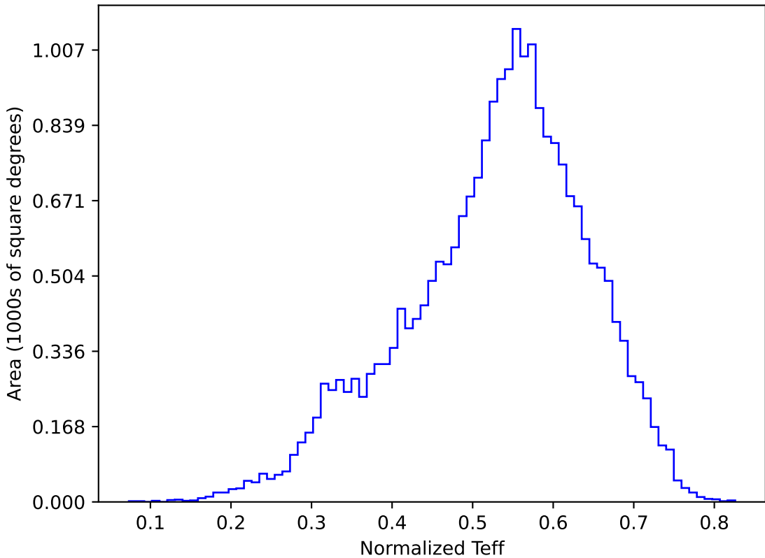
too_elab_r16_d3_giz_v3.4_10yrs All sky y band: Normalized Teff
