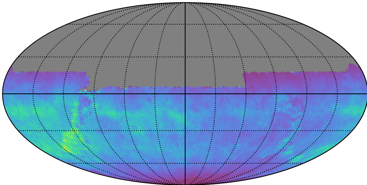
too_elab_r16_d3_giz_v3.4_10yrs All sky u band: Normalized Teff
