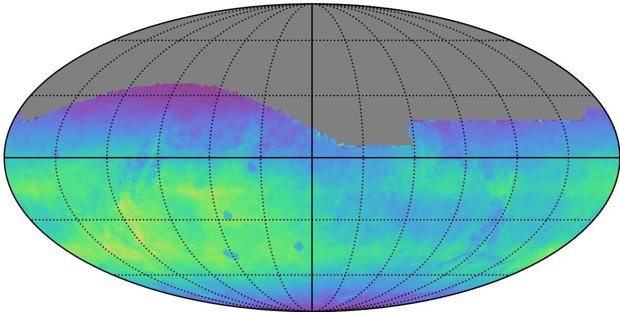
too_elab_r16_d3_giz_v3.4_10yrs All sky r band: Normalized Teff
