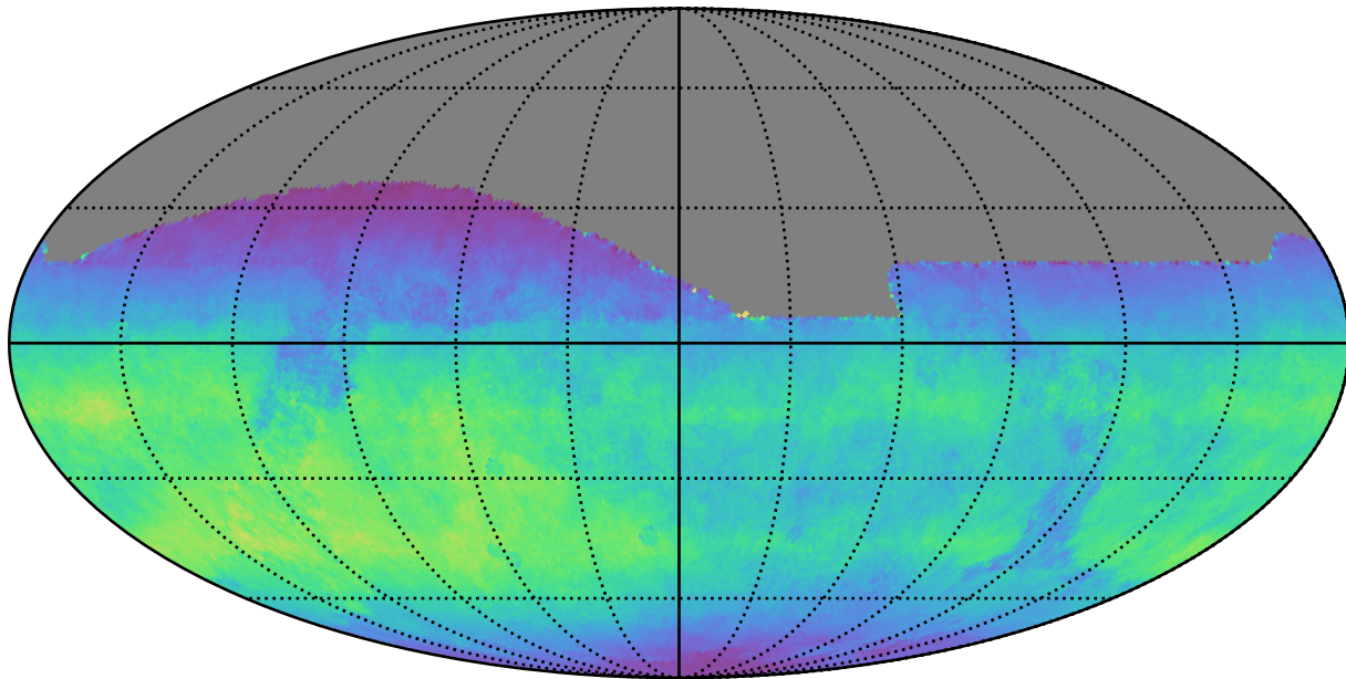
too_elab_r16_d3_giz_v3.4_10yrs All sky i band: Normalized Teff
