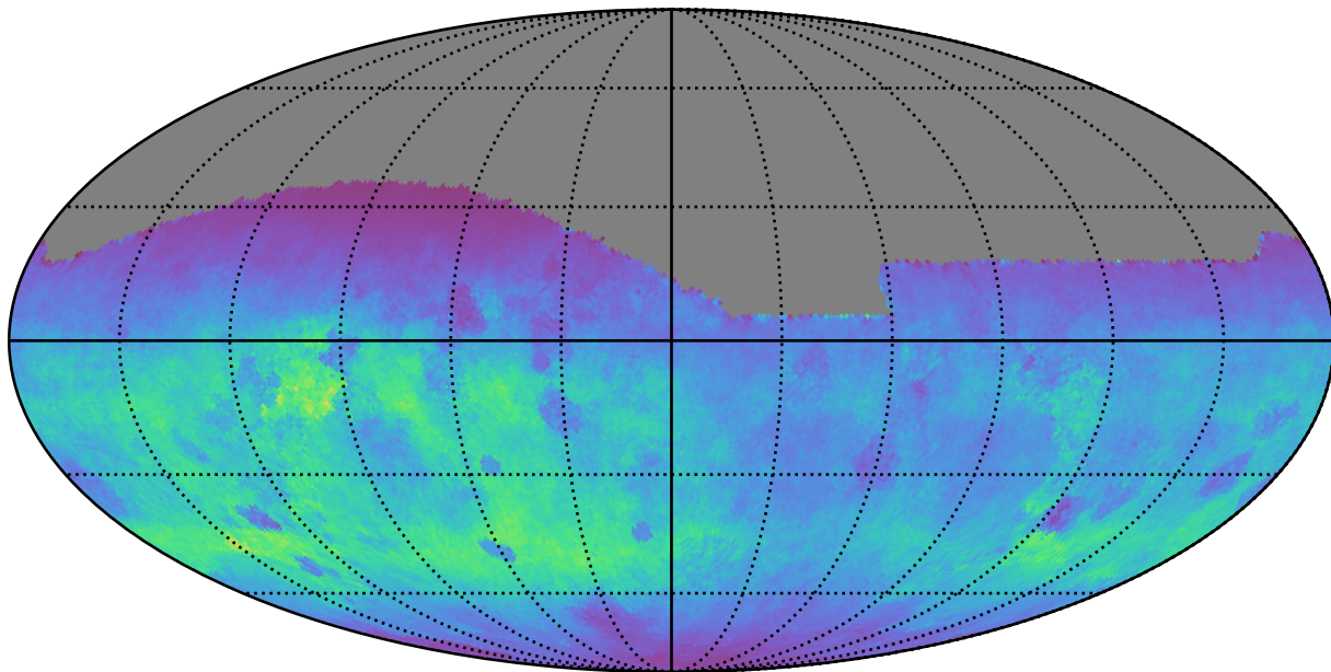
too_elab_r16_d3_giz_v3.4_10yrs All sky g band: Normalized Teff
