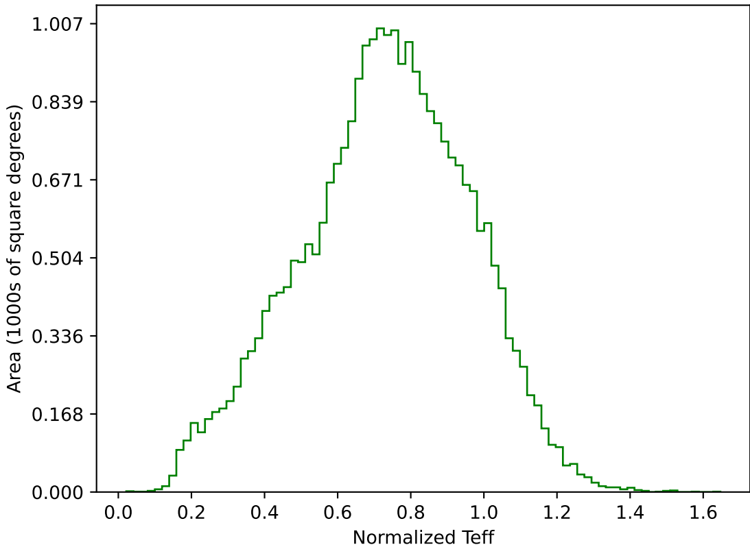
too_elab_r16_d3_giz_v3.4_10yrs All sky g band: Normalized Teff
