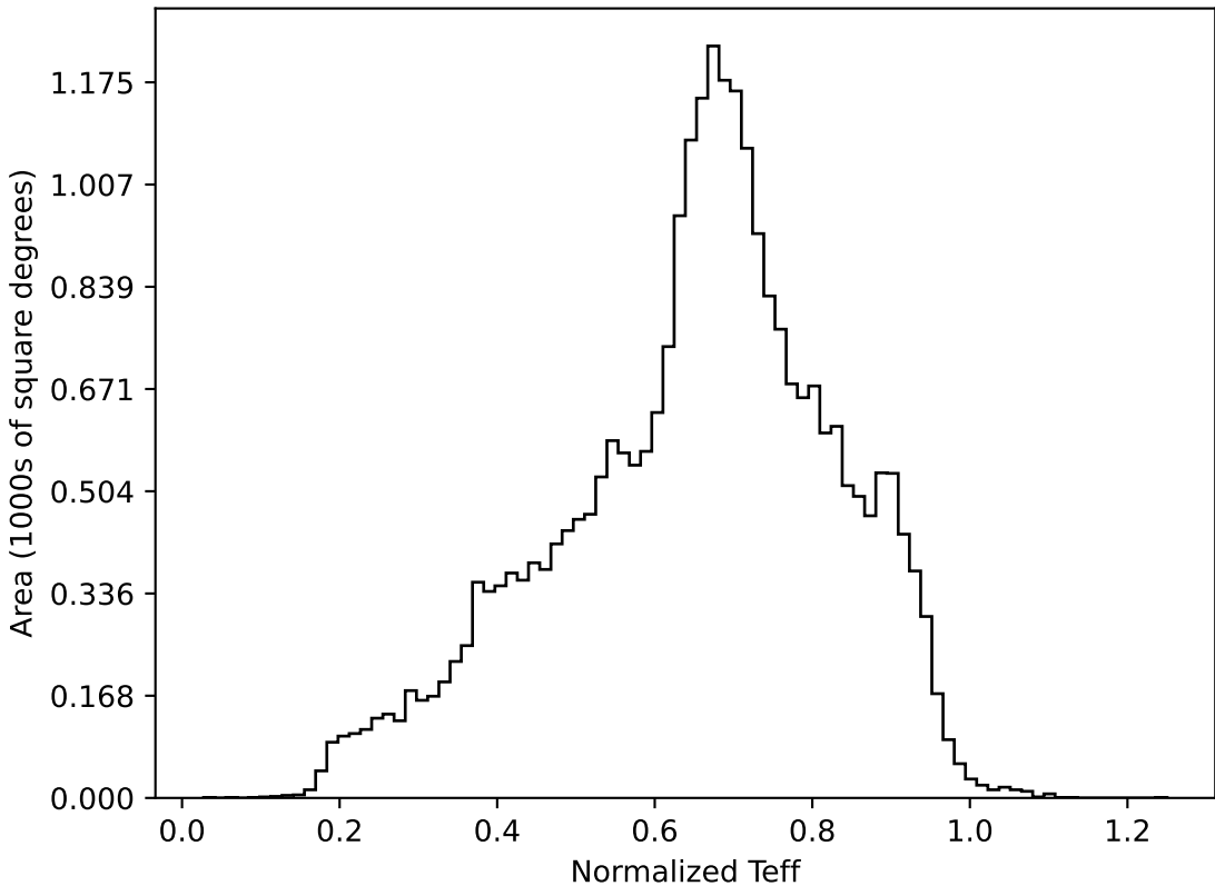
too_elab_r16_d3_giz_v3.4_10yrs All sky all bands: Normalized Teff
