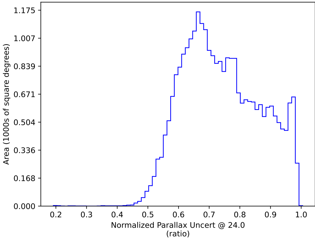
too_elab_r16_d3_giz_v3.4_10yrs All sky: Normalized Parallax Uncert @ 24.0
