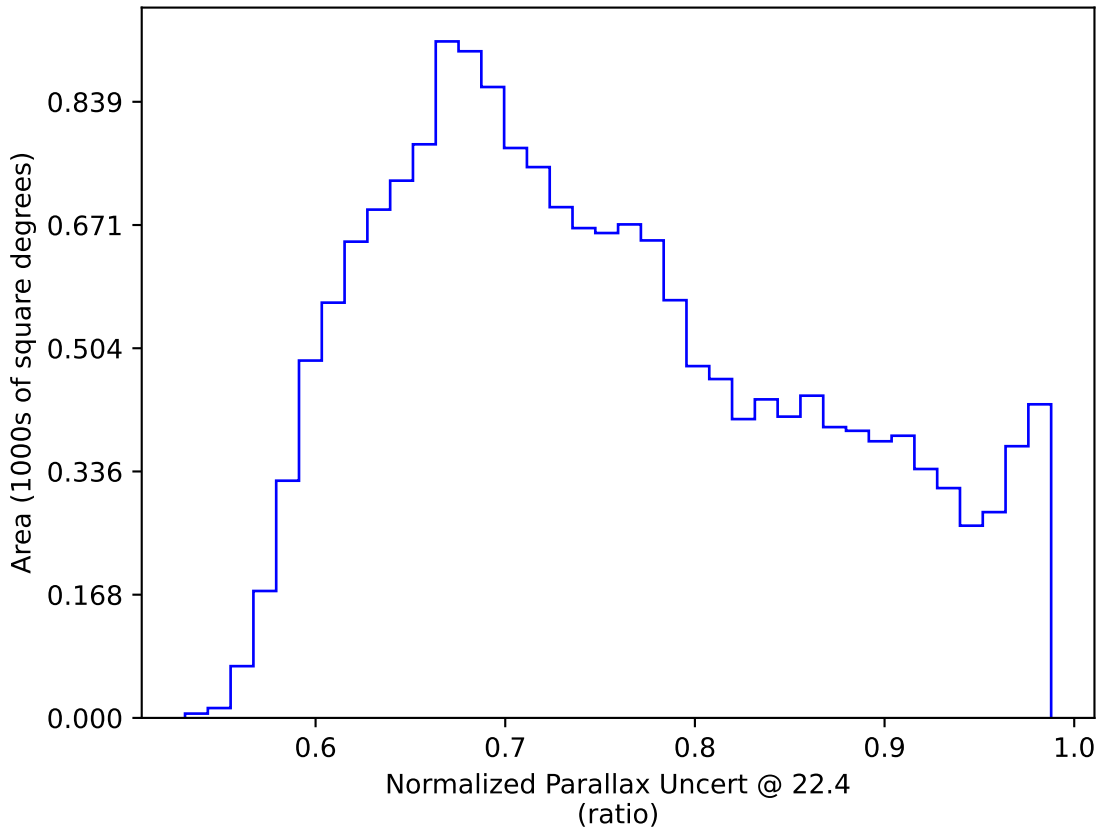
too_elab_r16_d3_giz_v3.4_10yrs WFD: Normalized Parallax Uncert @ 22.4
