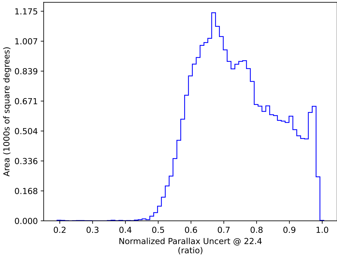
too_elab_r16_d3_giz_v3.4_10yrs All sky: Normalized Parallax Uncert @ 22.4
