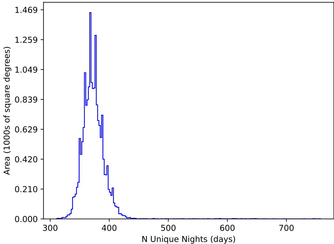
too_elab_r16_d3_giz_v3.4_10yrs WFD all bands: N Unique Nights
