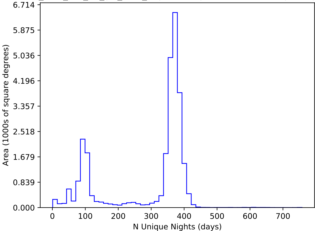
too_elab_r16_d3_giz_v3.4_10yrs All sky all bands: N Unique Nights
